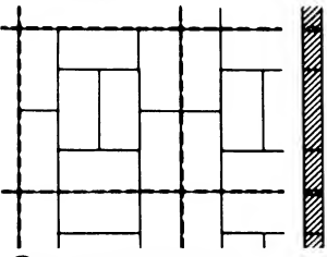
13 1/4 brick thick (brick on edge) reinforced wall with 8 brick panel
